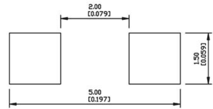
Recommended Soldering Pattern For Reflow Soldering
