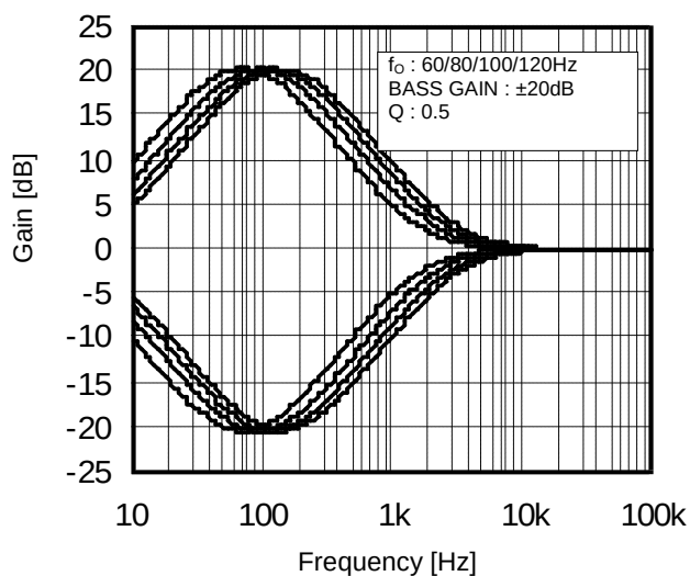
Figure 5. Bass fo vs Frequency
