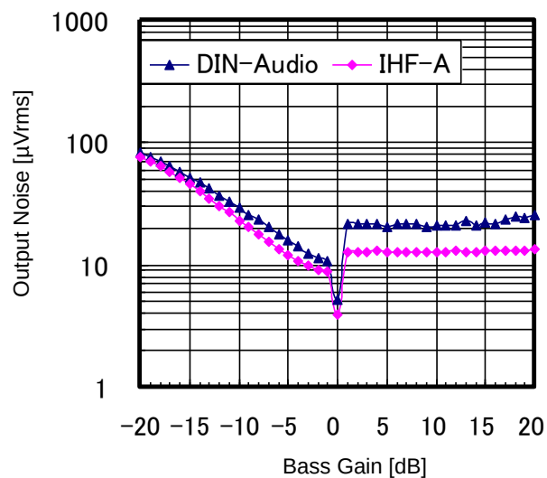
Figure 14. Output Noise vs Bass Gain
