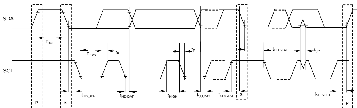
Figure 22. I 2 C-bus Signal Timing Diagram
