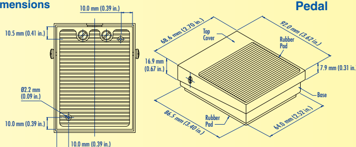
Pedal
