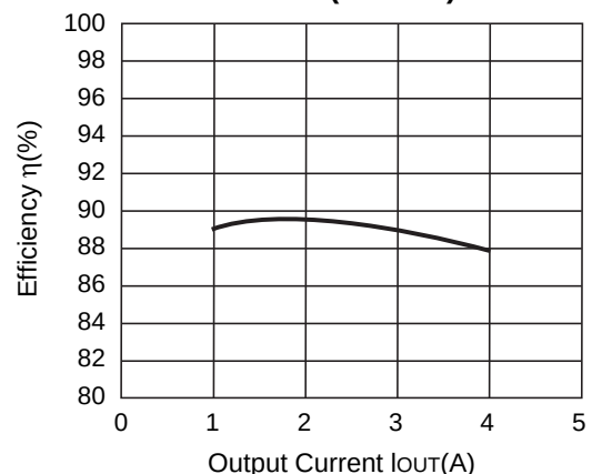
R1224N332M (V IN =10V)
