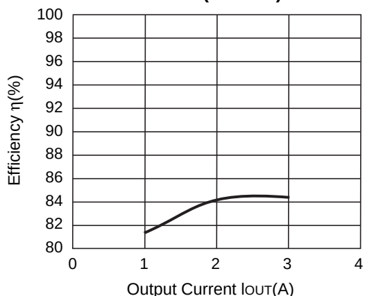
R1224N332M (V IN =18V)
