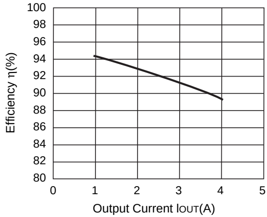
R1224N332M (V IN =5V)
