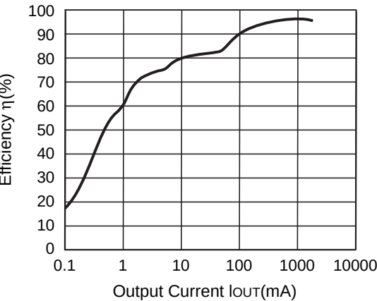
R1224N502E (V IN =6.5V) CDRH127-10μH
