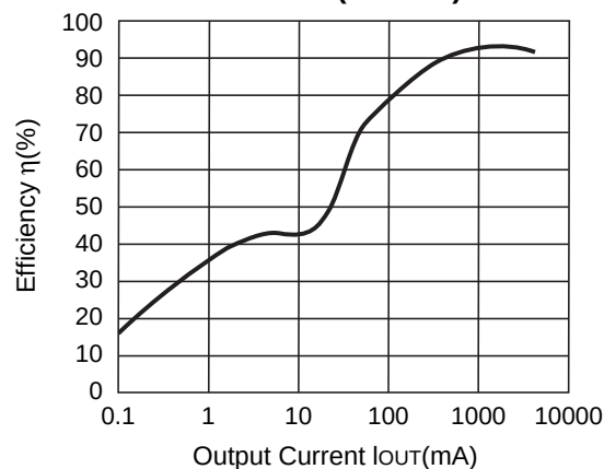
R1224N502G ( V_{IN}=10V )
