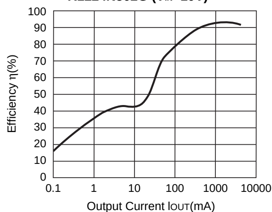
R1224N502G ( V_{IN}=10V )
