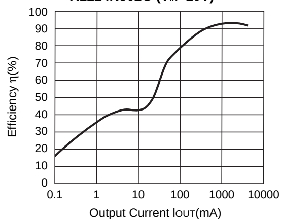
R1224N502G ( V_{IN}=10V )
