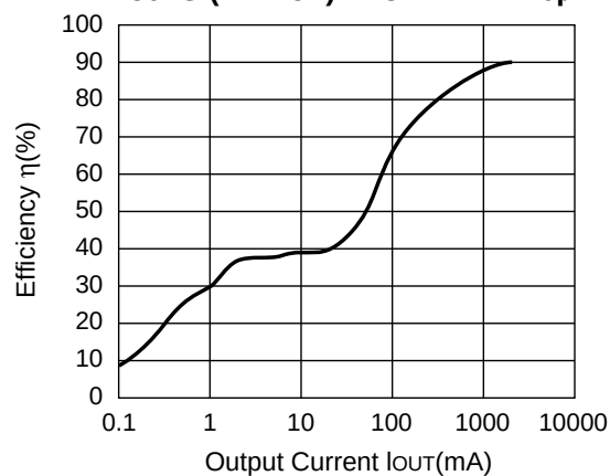
R1224N502G ( V_{IN}=15V ) CDRH127-10 \mu H
