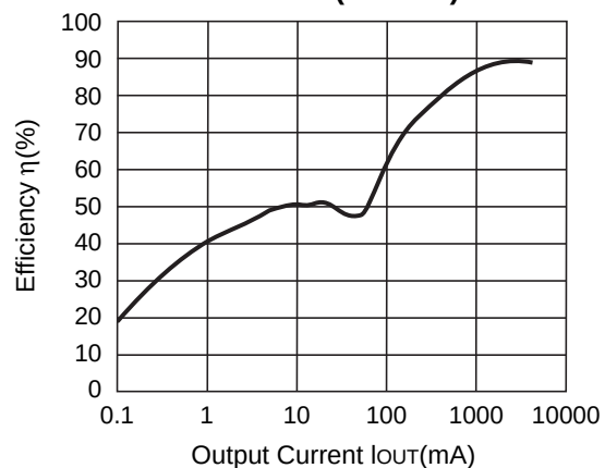
R1224N502G ( V_{IN}=16V )
