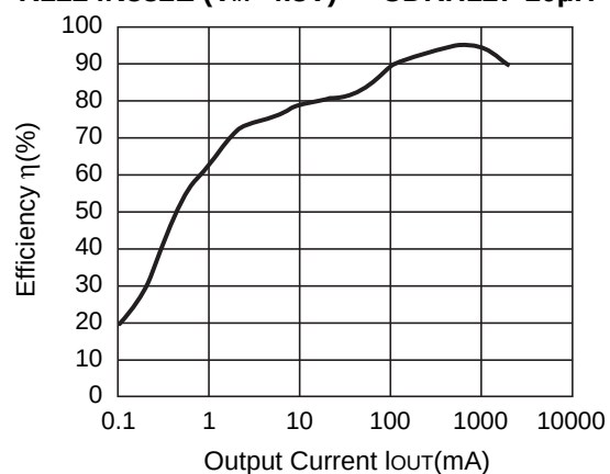
R1224N332E ( V_{IN}=4.8V ) CDRH127-10 \mu H
