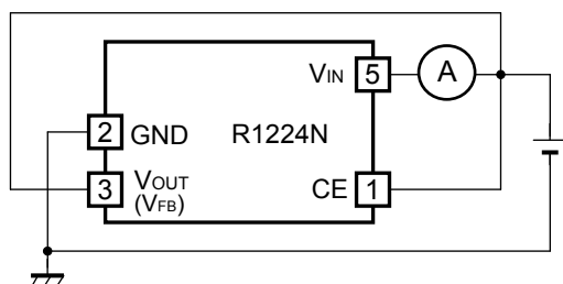
Supply Current 1
