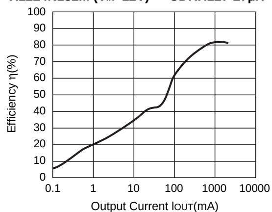
R1224N182M ( V_{IN}=12V ) CDRH127-27 \mu H
