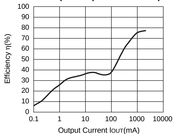
R1224N182H ( V_{IN}=12V ) CDRH127-10 \mu H
