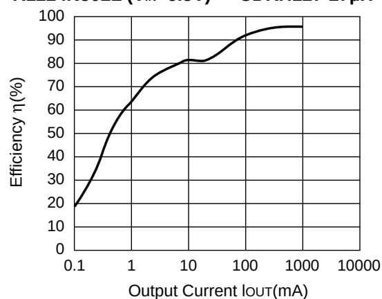
R1224N502L ( V_{IN}=6.5V ) CDRH127-27 \mu H
