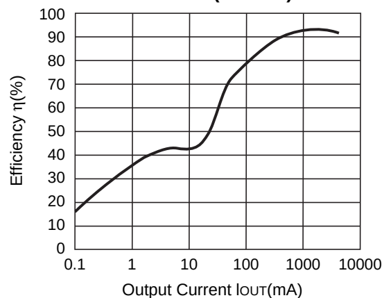
R1224N502G ( V_{IN}=10V )
