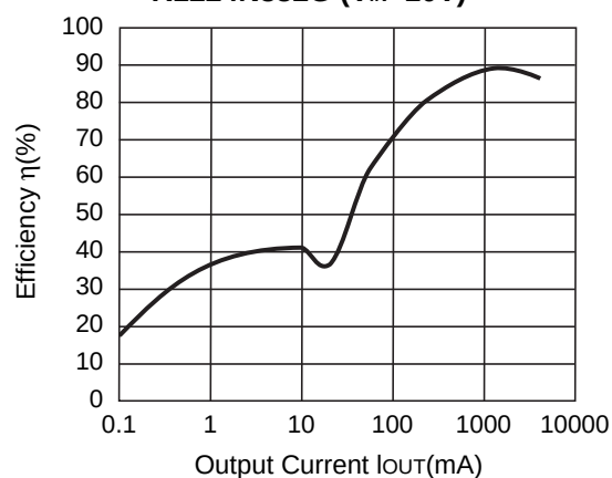
R1224N332G ( V_{IN}=10V )
