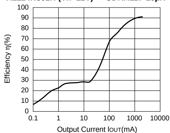
R1224N502H ( V_{IN}=12V ) CDRH127-10 \mu H
