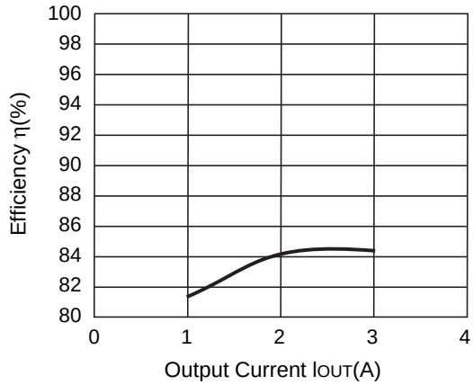
R1224N332M ( V_{IN}=18V )
