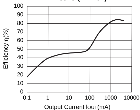
R1224N332G ( V_{IN}=16V )
