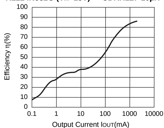
R1224N332G ( V_{IN}=15V ) CDRH127-10 \mu H
