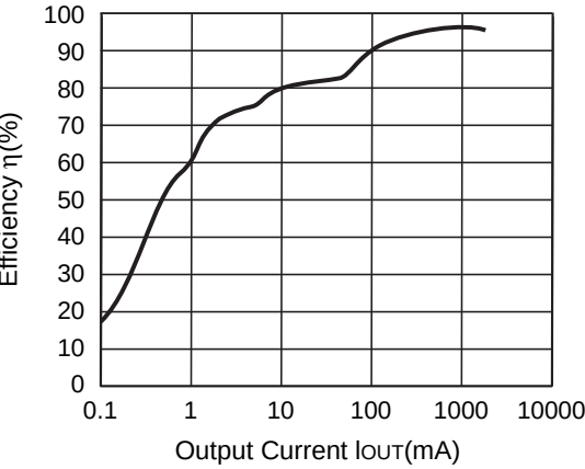
R1224N502E ( V_{IN}=6.5V ) CDRH127-10 \mu H
