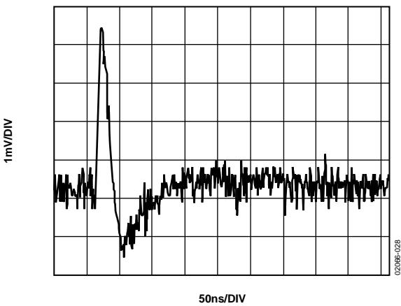
Figure 28. DAC-to-DAC Crosstalk
