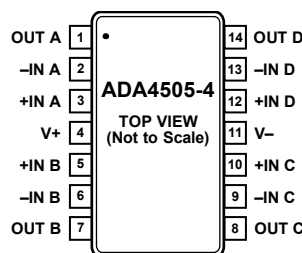
Figure 5. 14-Lead TSSOP (RU-14)
