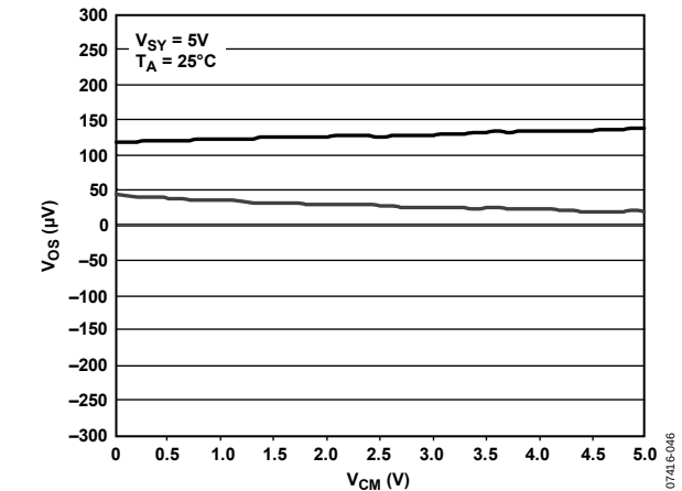
Figure 56. Input Offset Voltage vs. Input Common-Mode Voltage Response (Powered by a 5 V Supply; Results of Two Units Are Displayed)
