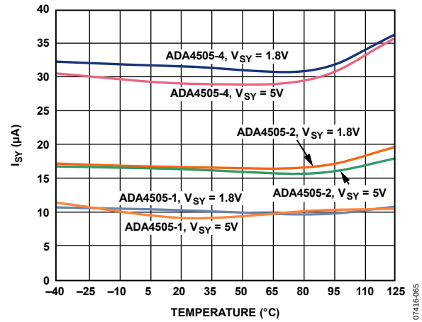
Figure 46. Total Supply Current vs. Temperature
