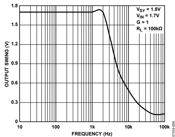
Figure 49. Output Swing vs. Frequency
