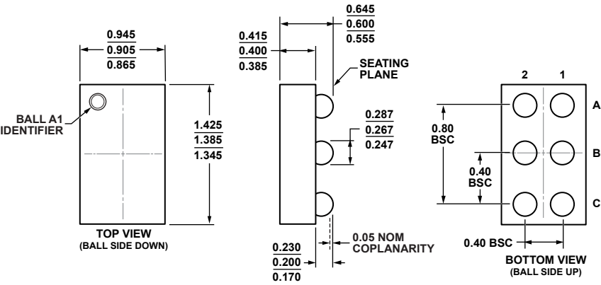
Figure 60. 6-Ball Wafer Level Chip Scale Package [WLCSP] (CB-6-7) Dimensions shown in millimeters
