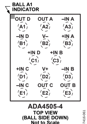
Figure 6. 14-Ball WLCSP (CB-14-1)
