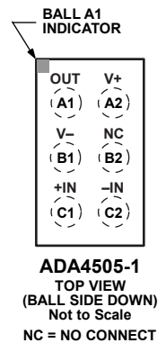
Figure 3. 6-Ball WLCSP (CB-6-7)
