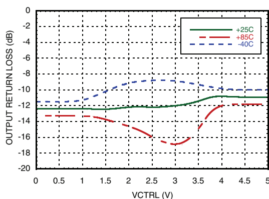
Output Return Loss vs. VCTRL @ 500MHz [1]
