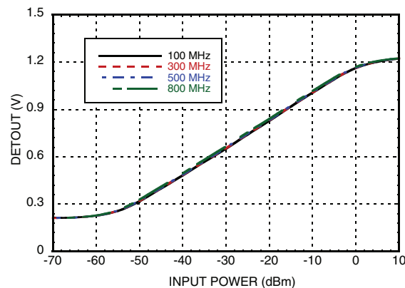
Figure 8: DETOUT vs. input power over frequency.
