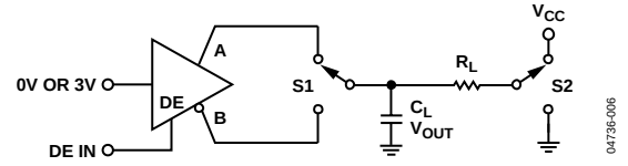
Figure 6. Driver Enable/Disable
