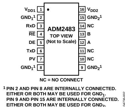
Figure 2. Pin Configuration
