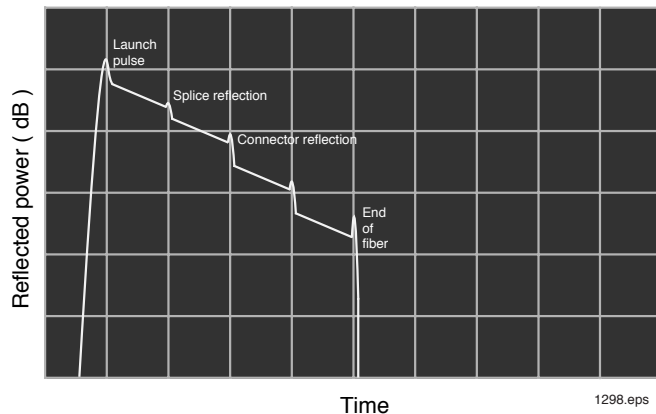
Figure 27. Typical display from an OTDR.
