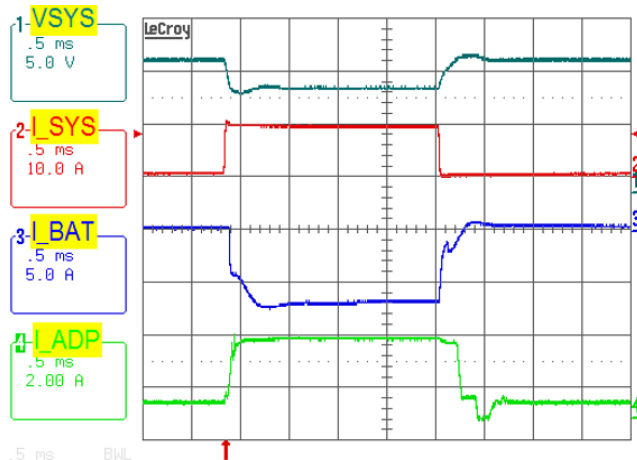
FIGURE 12. BUCK-BOOST MODE, OUTPUT VOLTAGE LOOP TO ADAPTER CURRENT LOOP TRANSITION. V_{ADP} = 12V , MAXSYSTEMVOLTAGE = 12.576V , V_{BAT} = 11V , SYSTEM LOAD 1A TO 10A STEP, ADAPTERCURRENTLIMIT = 3A , CHARGECURRENT = 0A
