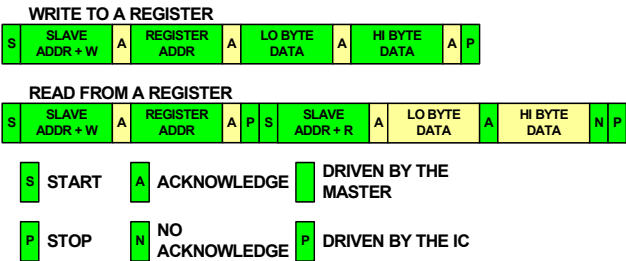
FIGURE 24. SMBus READ AND WRITE PROTOCOL
