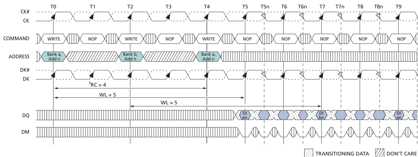
Figure 21: Consecutive WRITE-to-WRITE
