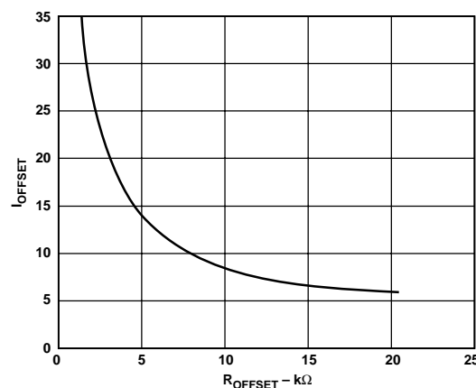
Figure 2. I_{\text{OFFSET}} vs. R_{\text{OFFSET}}
