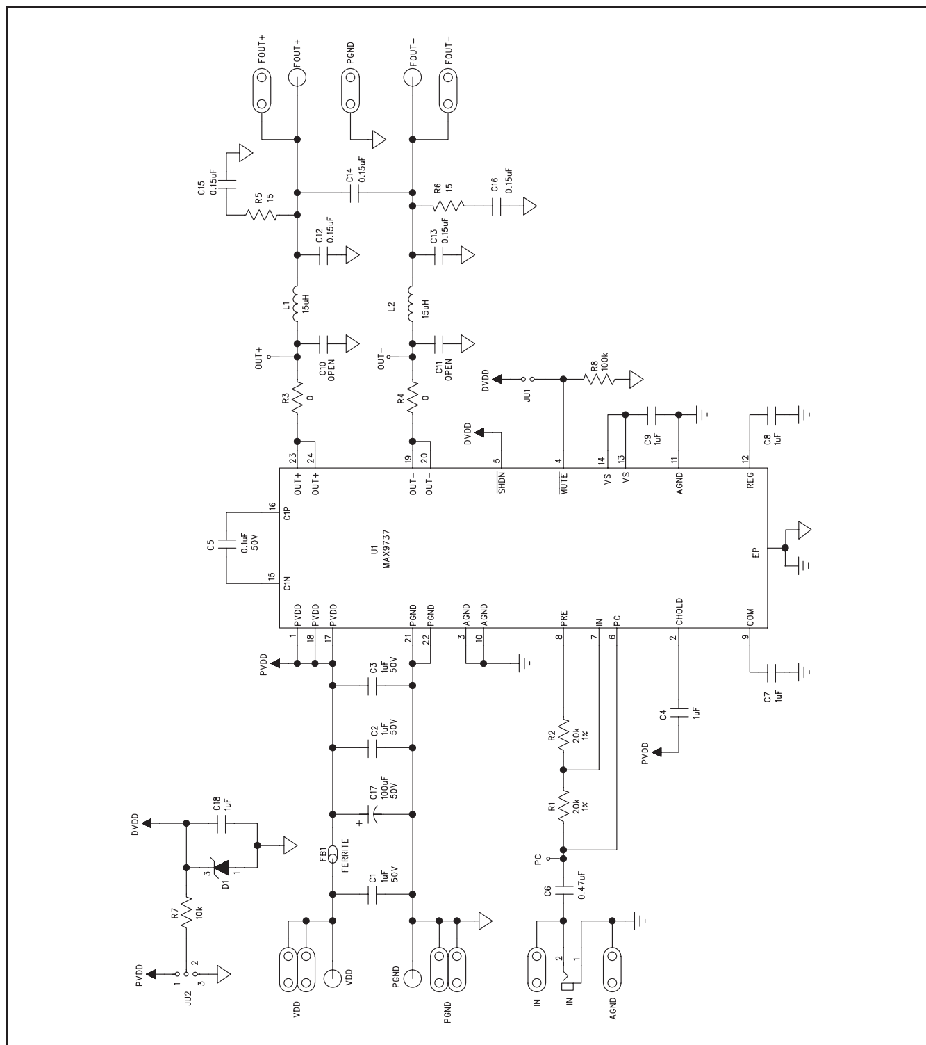
Figure 1. MAX9737 EV Kit Schematic
