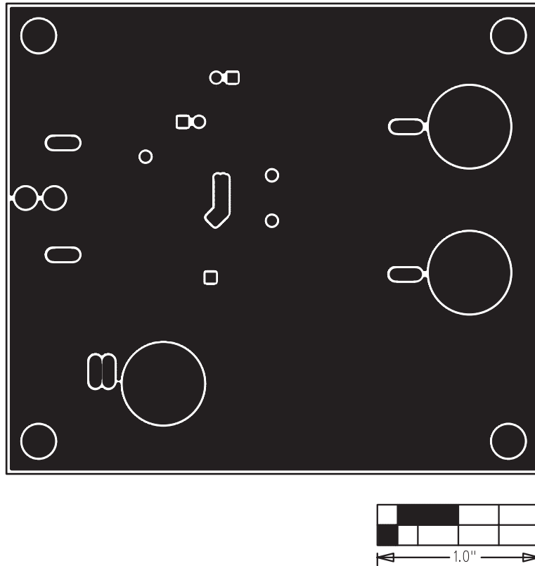
Figure 4. MAX9737 EV Kit PCB Layout—Solder Side
