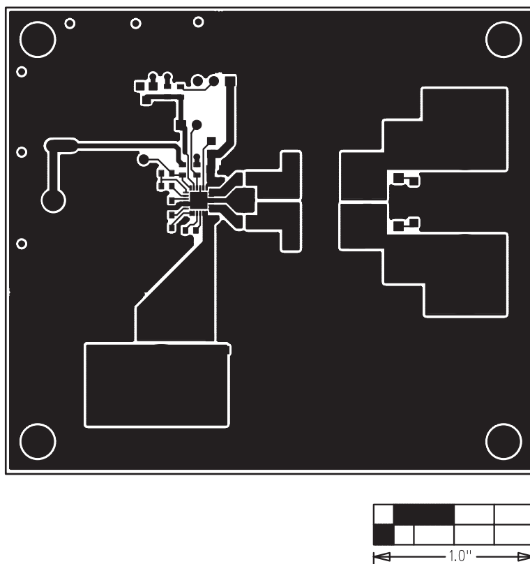
Figure 3. MAX9737 EV Kit PCB Layout—Component Side
