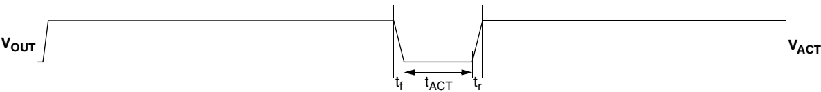
Fig. 5-4: Activate pulse
