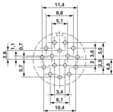
Drilling diagram
