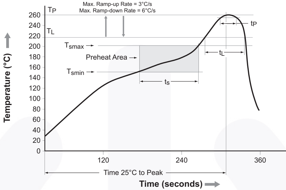
Figure 17. Reflow Profile
