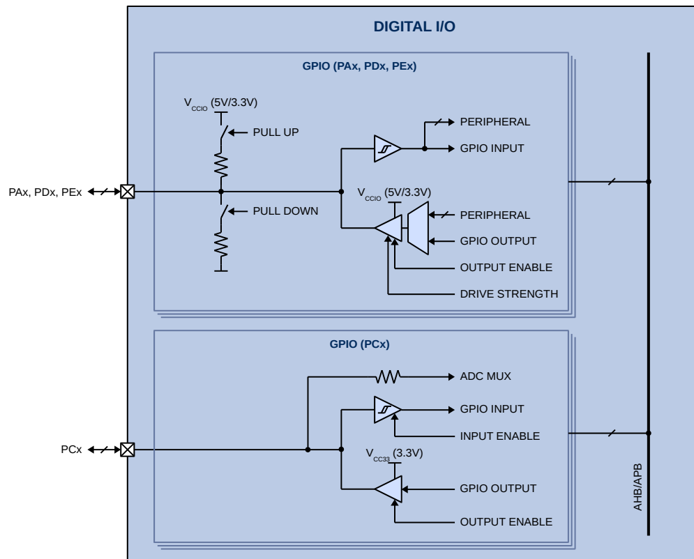
Figure 17-1 I/O controller
