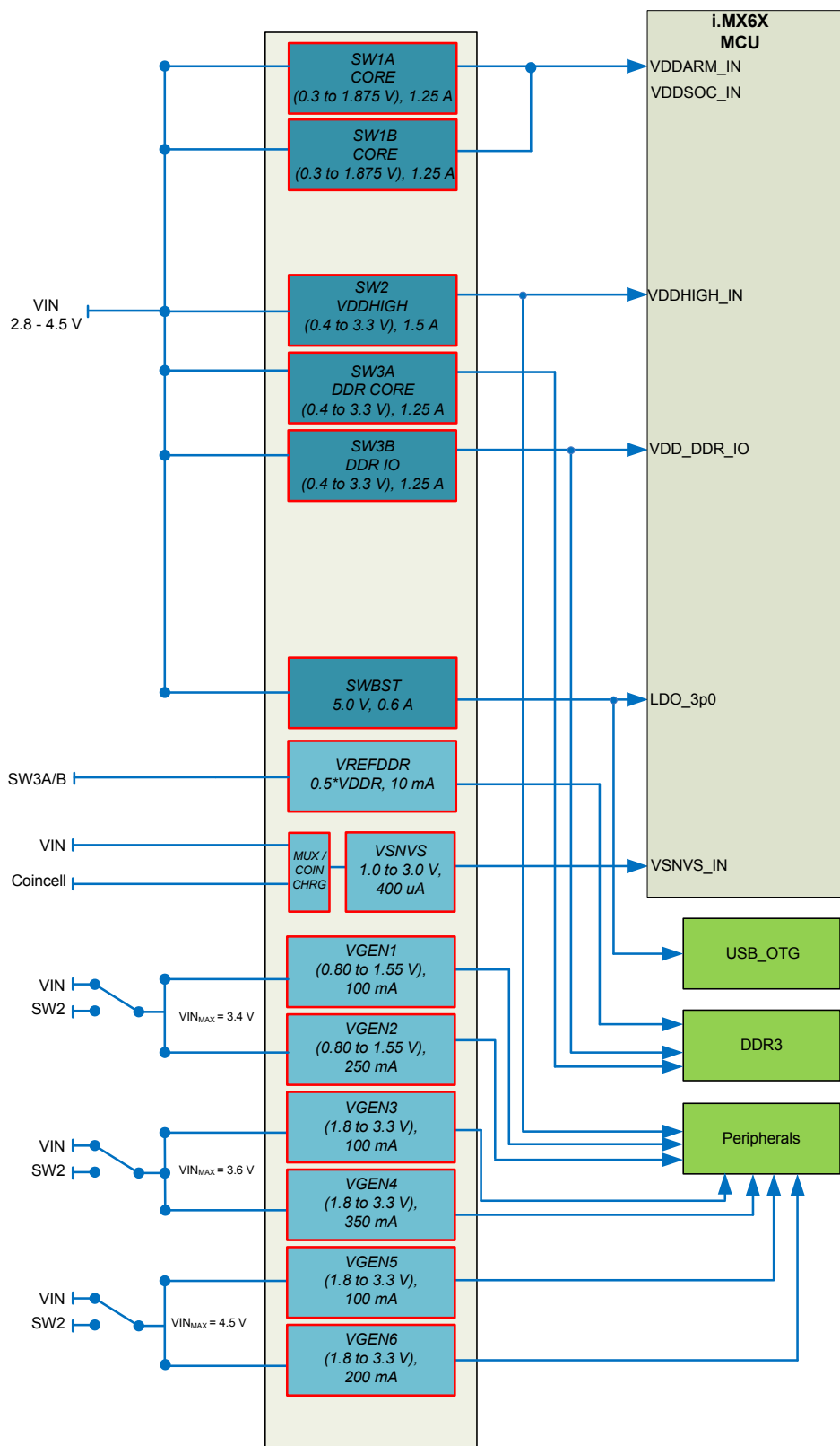
Figure 9. PF0200Z Typical Power Map
