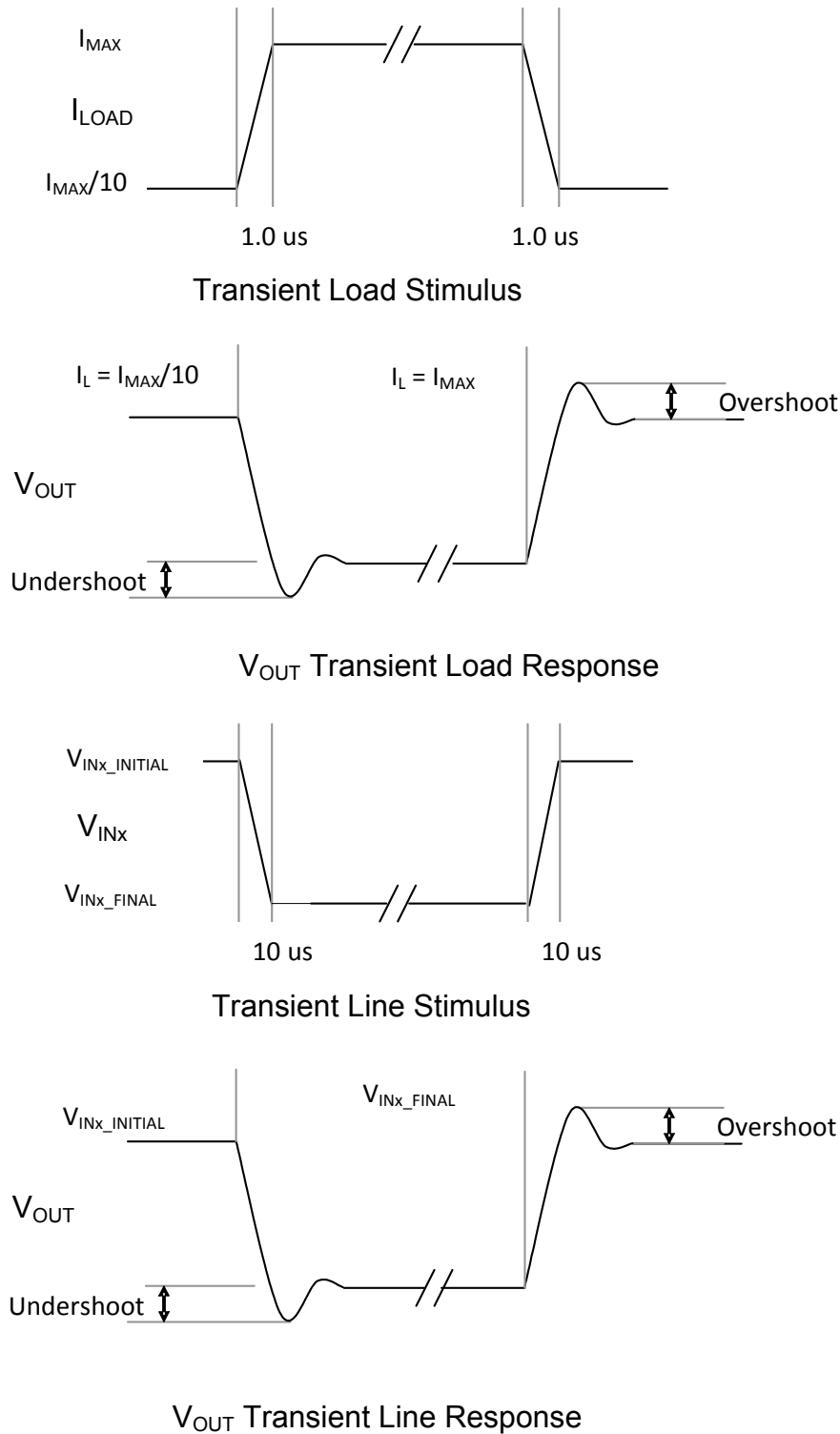
Figure 20. Transient Waveforms
