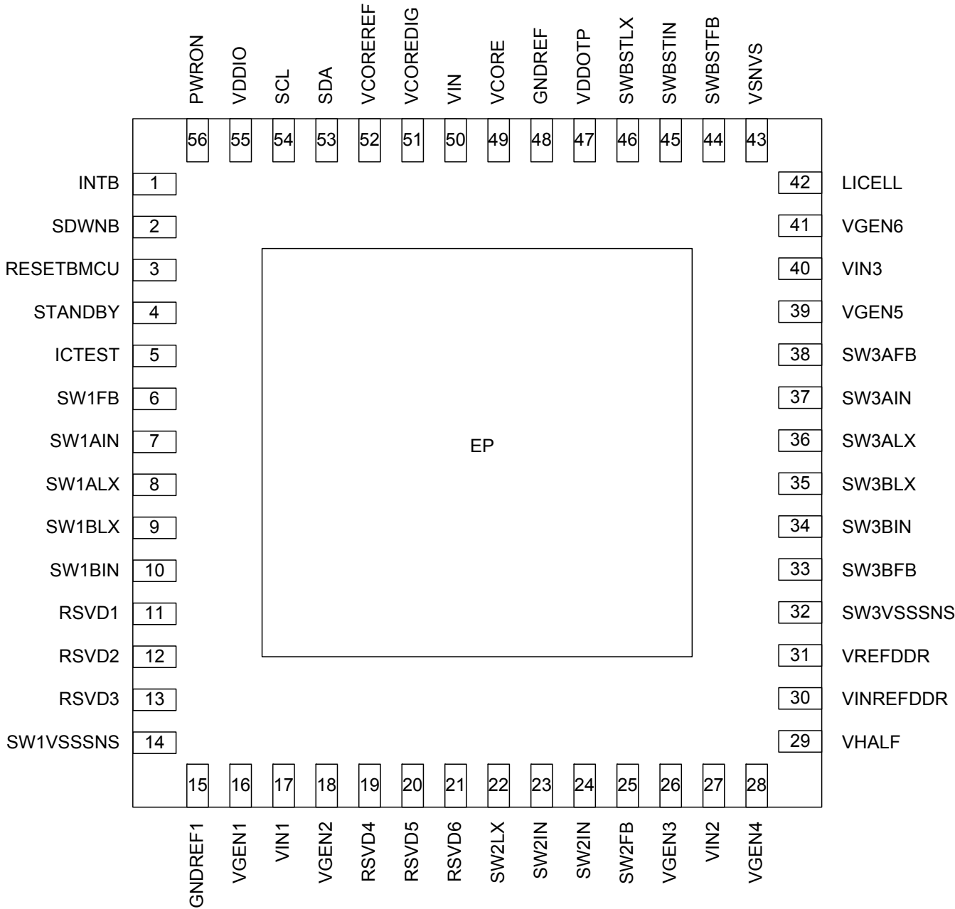
Figure 3. Pinout Diagram
