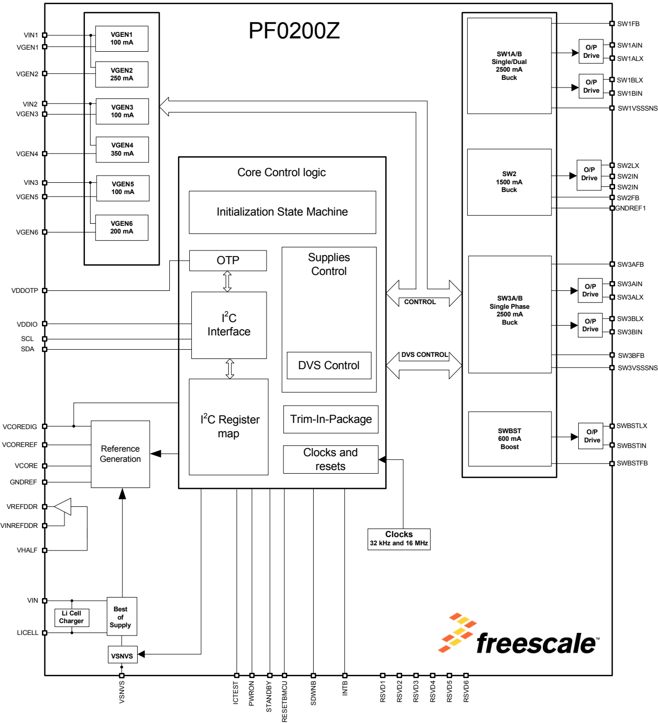
Figure 2. Simplified Internal Block Diagram
