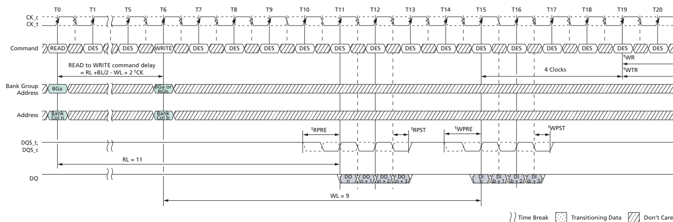
Figure 144: READ (BC4) OTF to WRITE (BC4) OTF with 1 st CK Preamble in Same or Different Bank Group
