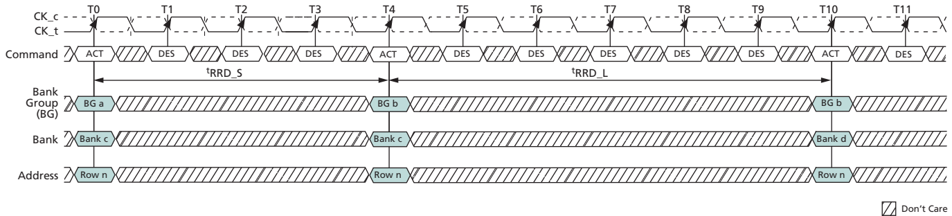
Figure 81: t_{RRD} Timing
