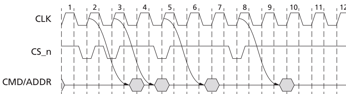
Figure 27: CAL Timing Example (Consecutive CS n = LOW)
