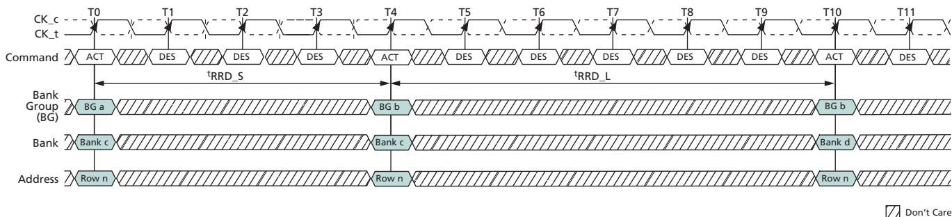
Figure 81: t_{RRD} Timing
