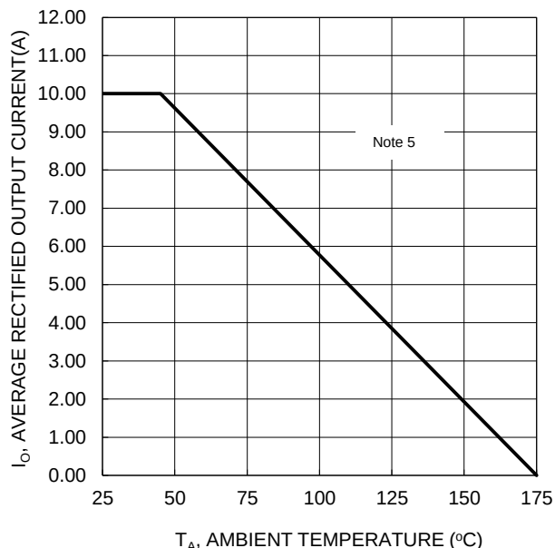
Figure 4 DC Forward Current Derating
