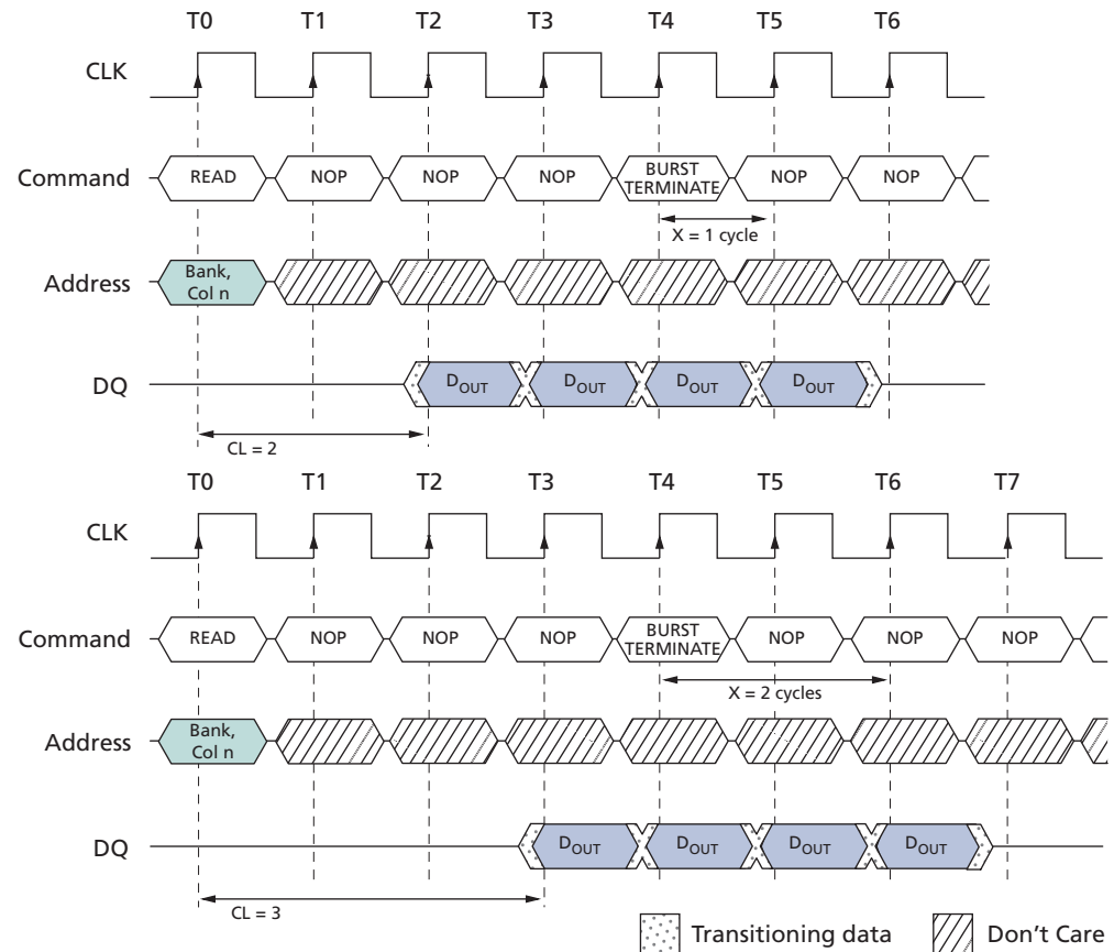
Figure 26: Terminating a READ Burst
