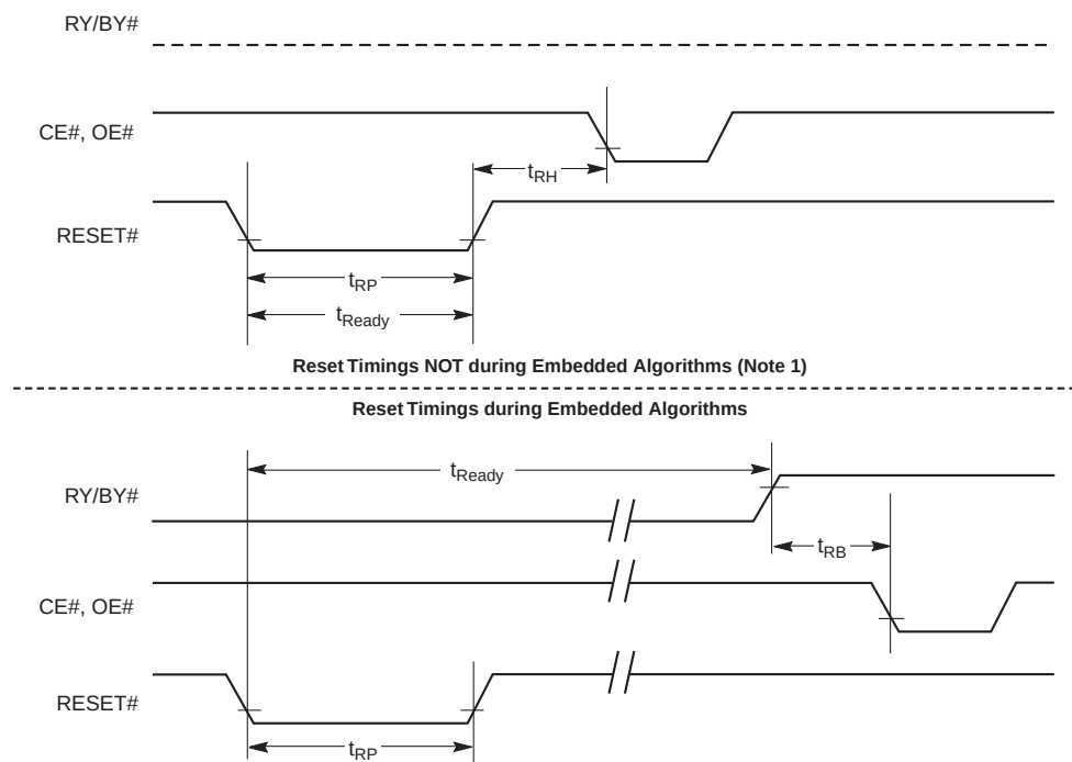
Figure 15. RESET# Timings
