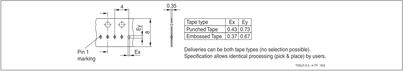
Figure 12 TSSLP-2-4 packing
