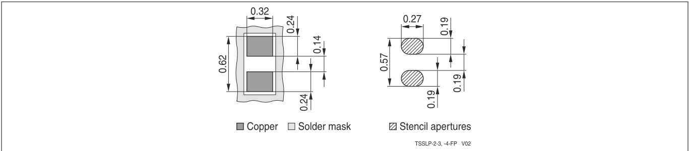
Figure 11 TSSLP-2-4 footprint
