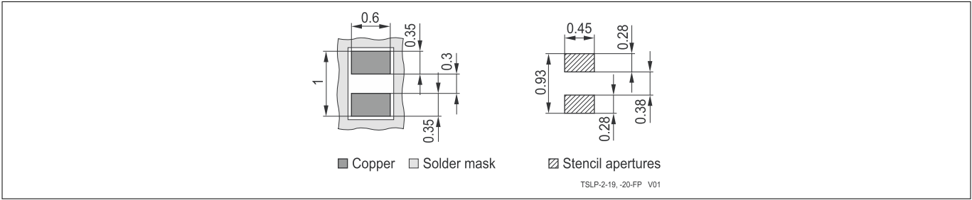
Figure 15 TSLP-2-20 footprint
