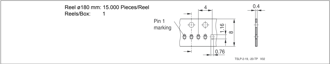
Figure 16 TSLP-2-20 packing
