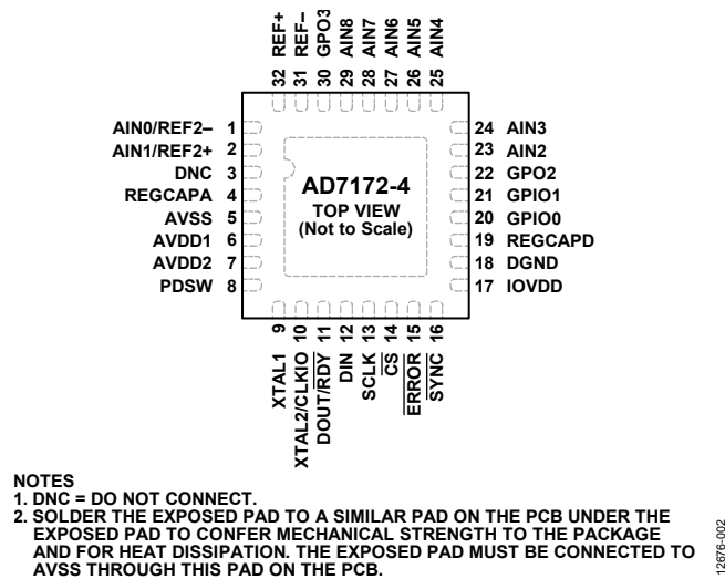
Figure 4. Pin Configuration
