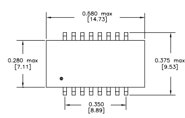
N6 Package
