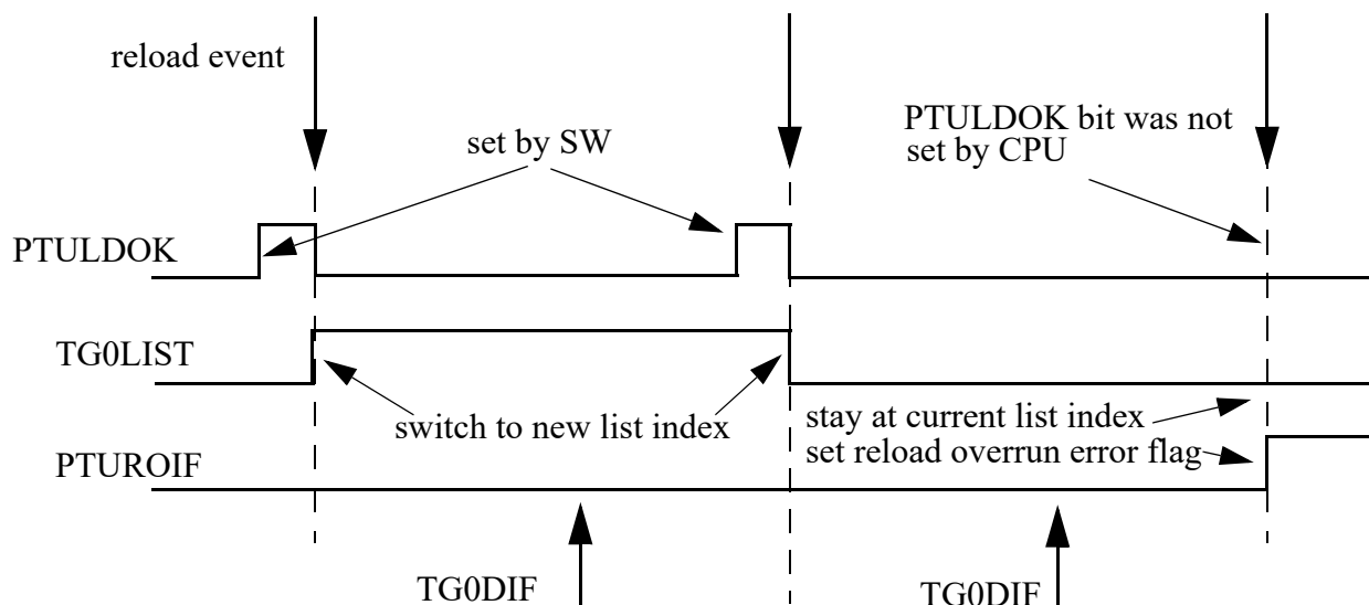
Figure 13-19. TG0 Reload behavior with local PTULDOK
