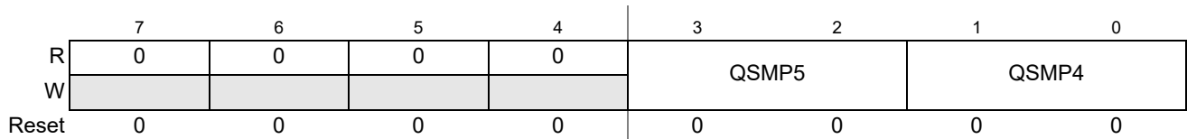
Figure 12-11. PMF Fault Qualifying Samples Register (PMFQSMP0)
