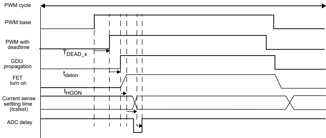
Figure 1-11. Control Loop Delay Overview
