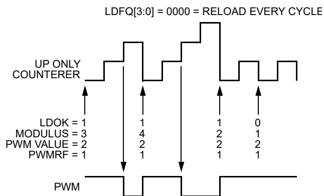
Figure 12-81. Edge-Aligned Modulus Loading
