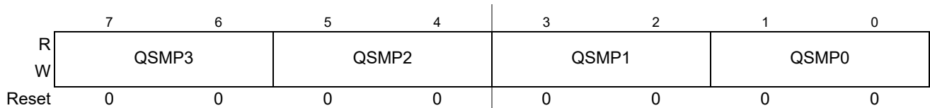
Figure 12-12. PMF Fault Qualifying Samples Register (PMFQSMP1)
