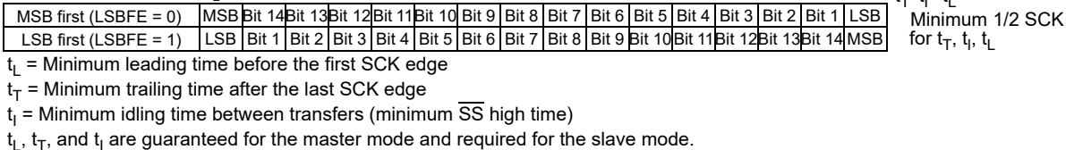
Figure 15-13. SPI Clock Format 0 (CPHA = 0), with 16-Bit Transfer Width selected (XFRW = 1)
