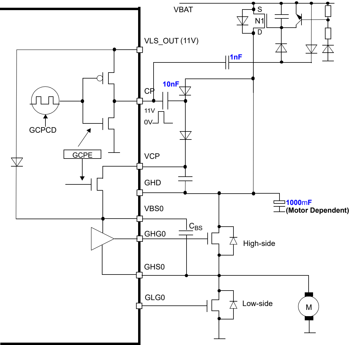
Figure 1-13. High-side Supply and Charge Pump Concept
