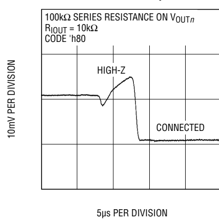
Voltage Buffered IDAC Soft-Connect Transient Response
