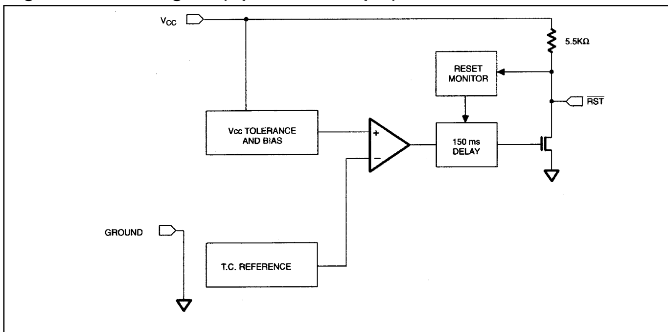
Figure 1. Block Diagram (Open-Drain Output)
