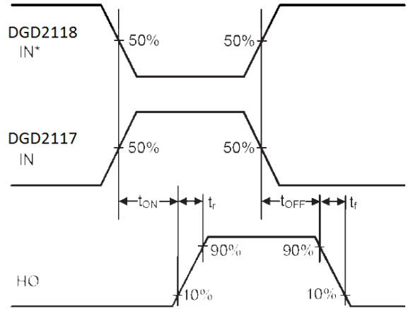
Figure 2. Switching Time Waveform Definitions
