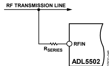
Figure 46. Attenuating the Input Signal
