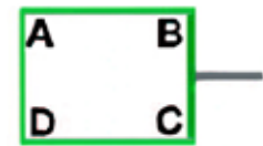
Origin (0,0) Point
