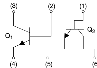
MBT3904DW2T1 STYLE 27
