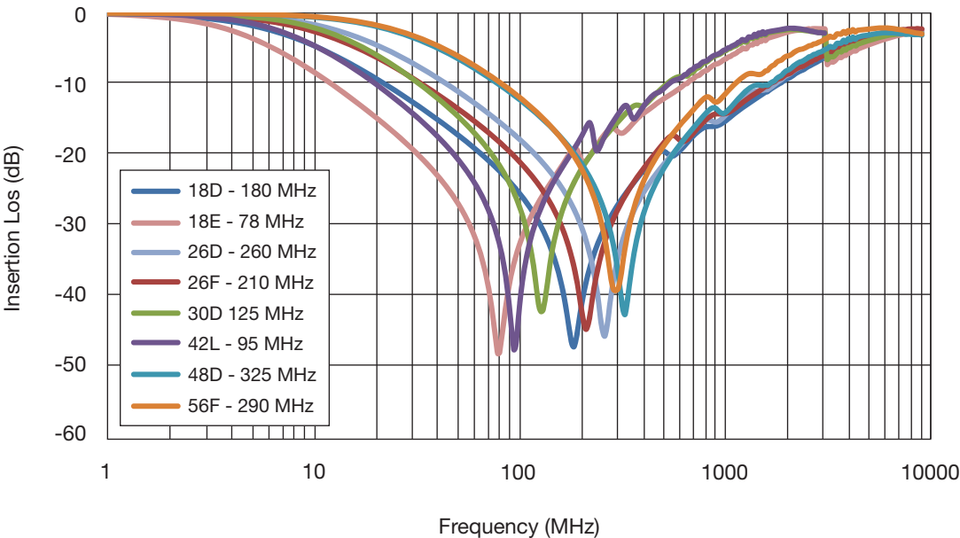
1206 Case Size
