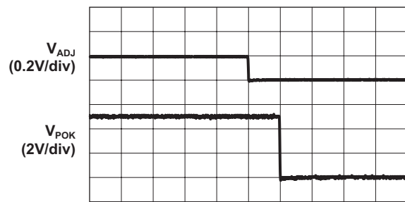
ADJ Detect Delay Time ( V_{CC} = 5.0V , R_{SET} = 1.24M\Omega , V_{ADJ} = 1.3V to 1.1V )
