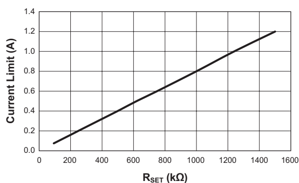
Current Limit vs. R_{SET} ( V_{CC} = 5.0V )
