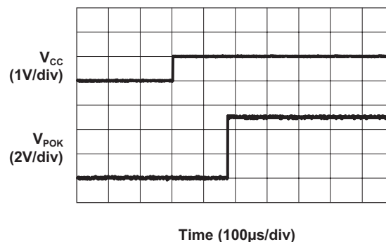
POK Delay Time ( R_{ADJ} = 18.2k\Omega , V_{CC} = 4V to 5V)
