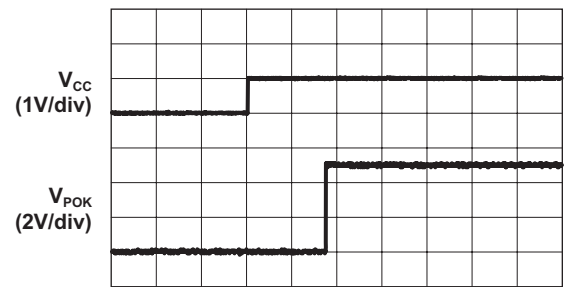
POK Delay Time ( R_{ADJ} = 18.2k\Omega , V_{CC} = 4V to 5V )
