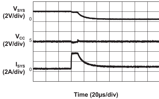
Current Limit Response ( V_{CC} = 5.0V , R_{SET} = 1.24M\Omega , R_{LOAD} = 10\Omega to 1\Omega )
