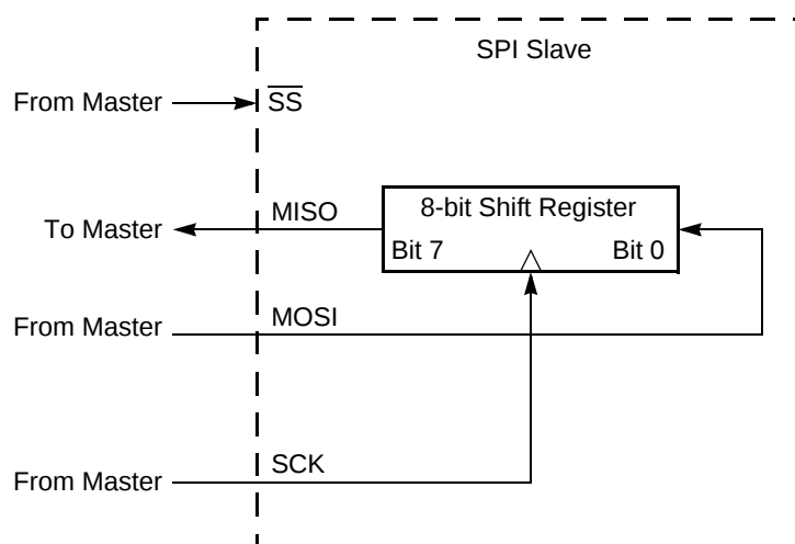
Figure 41. ESPI Configured as an SPI Slave
