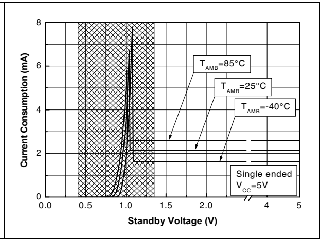
Figure 75. Current consumption vs. standby voltage, V CC = 5 V, SE
