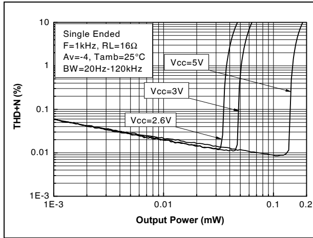
Figure 20. THD+N vs. output power, SE, F = 1 kHz, R_L = 16 \Omega , A_v = 4
