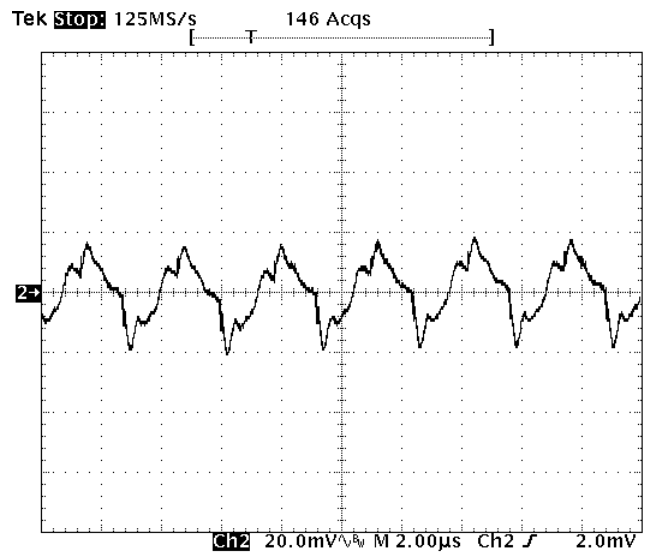
Fig-5.0V-5: Output voltage ripple (20mV/div.) for V_{out}=5.0V at full rated load current into a resistive load with external capacitance 47\mu F \times 4 ceramic + 1\mu F ceramic at V_{in}=12V . Time scale: 2 us/div
