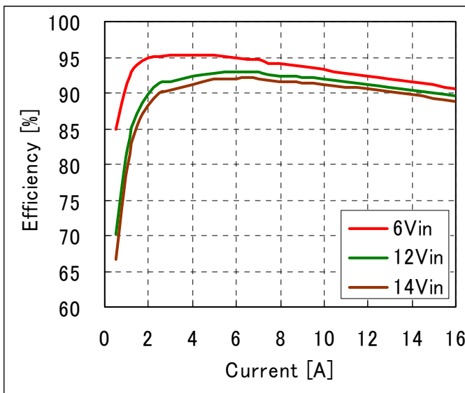
Fig-2.5V-2: Efficiency vs. load current and input voltage for Vout=2.5V. Airflow rate=200 LFM (1m/s) and Ta=25°C.
