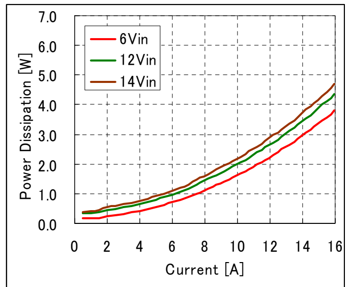
Fig-1.5V-3: Power Loss vs. load current and input voltage for Vout=1.5V. Airflow rate=200 LFM (1m/s) and Ta=25°C.
