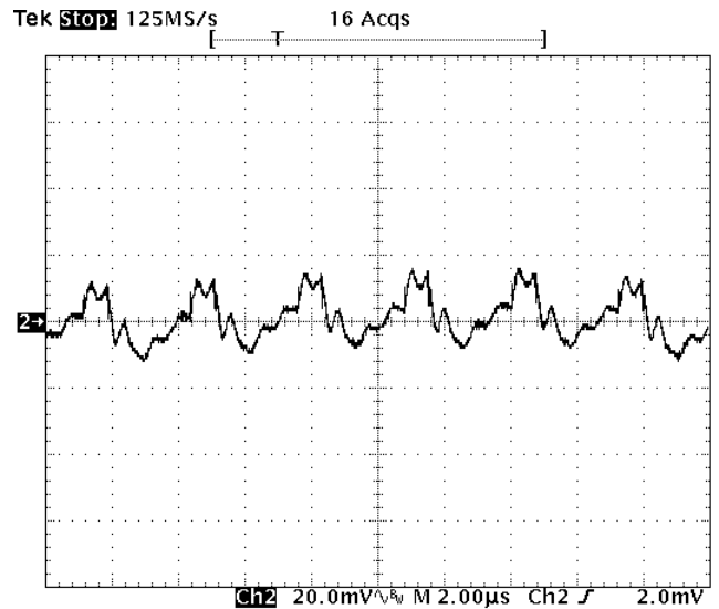
Fig-2.5V-5: Output voltage ripple (20mV/div.) for V_{out}=2.5V at full rated load current into a resistive load with external capacitance 47\mu F \times 4 ceramic + 1\mu F ceramic at V_{in}=12V . Time scale: 2 us/div
