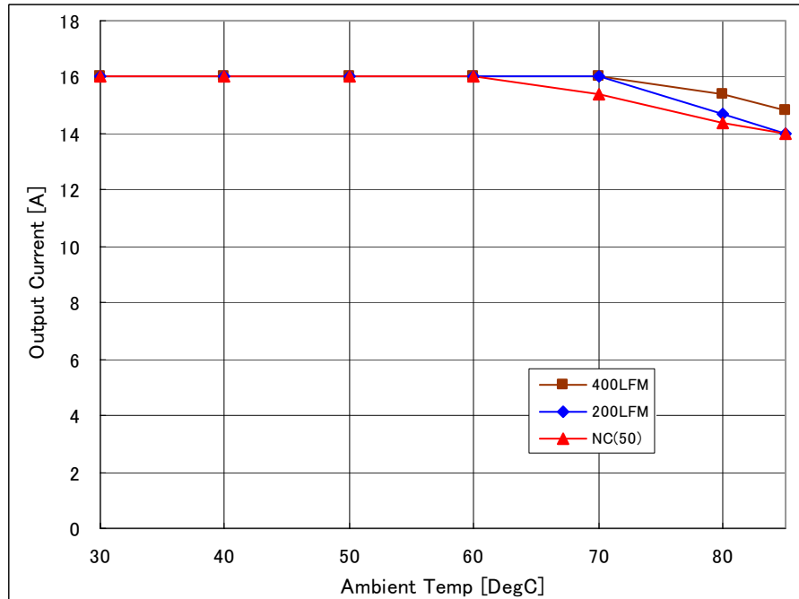
Fig-2.5V-1: Available load current vs. ambient temperature and airflow rates for Vout=2.5V with Vin=12V. Maximum component temperature ≤ 120°C
