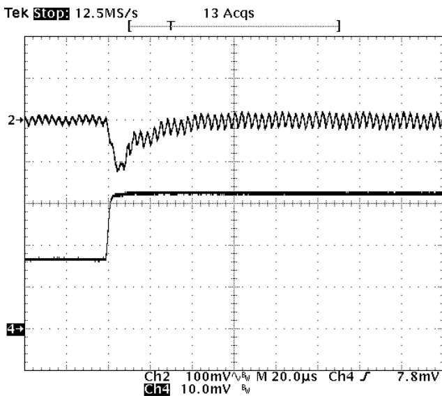
Fig-5.0V-6: Output voltage response for V_{out}=5.0V to positive load current step change from 8A to 16A with slew rate of 5A/\mu s at V_{in}=12V . C_o=47\mu F \times 4 ceramic. Top trace: output voltage (100mV/div.) Bottom trace: load current (5A/div.) Time scale: 20us/div.
