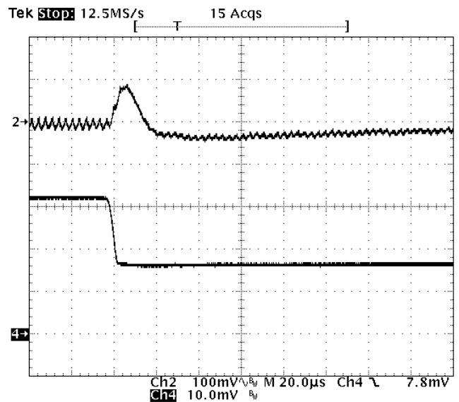
Fig-2.5V-7: Output voltage response for V_{out}=2.5V to negative load current step change from 16A to 8A with slew rate of -5A/\mu s at V_{in}=12V . C_o=47\mu F \times 4 ceramic. Top trace: output voltage (100mV/div.) Bottom trace: load current (5A/div.) Time scale: 20us/div.
