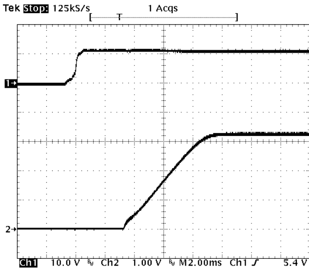
Fig-3.3V-4: Turn-on transient for V_{out}=3.3V with application of V_{in} at full rated load current (resistive) and 47uF \times 4 external capacitance at V_{in}=12V . Top trace: V_{in} (10V/div.) Bottom trace: output voltage (1V/div.) Time scale: 2ms/div.
