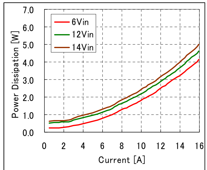
Fig-2.5V-3: Power Loss vs. load current and input voltage for Vout=2.5V. Airflow rate=200 LFM (1m/s) and Ta=25°C.
