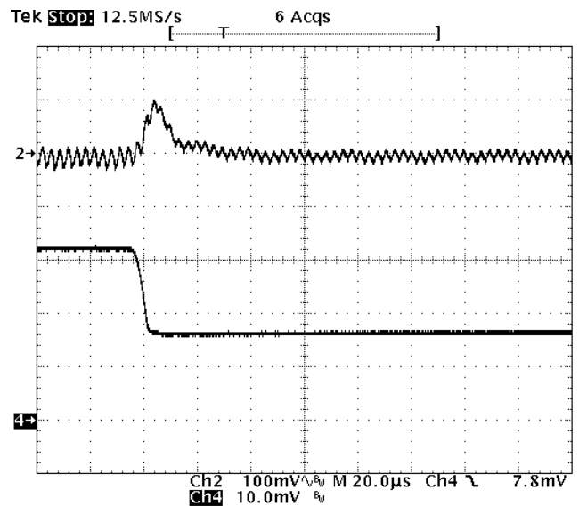
Fig-5.0V-7: Output voltage response for V_{out}=5.0V to negative load current step change from 16A to 8A with slew rate of -5A/\mu s at V_{in}=12V . C_o=47\mu F \times 4 ceramic. Top trace: output voltage (100mV/div.) Bottom trace: load current (5A/div.) Time scale: 20us/div.
