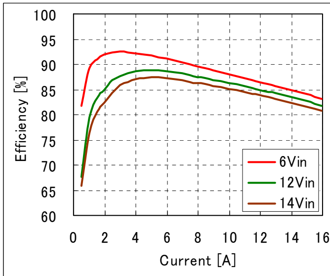
Fig-1.2V-2: Efficiency vs. load current and input voltage for V_{out}=1.2V . Airflow rate=200 LFM (1m/s) and T_a=25^{\circ}C .
