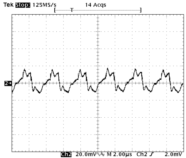
Fig-3.3V-5: Output voltage ripple (20mV/div.) for V_{out}=3.3V at full rated load current into a resistive load with external capacitance 47uF \times 4 ceramic + 1uF ceramic at V_{in}=12V . Time scale: 2 us/div
