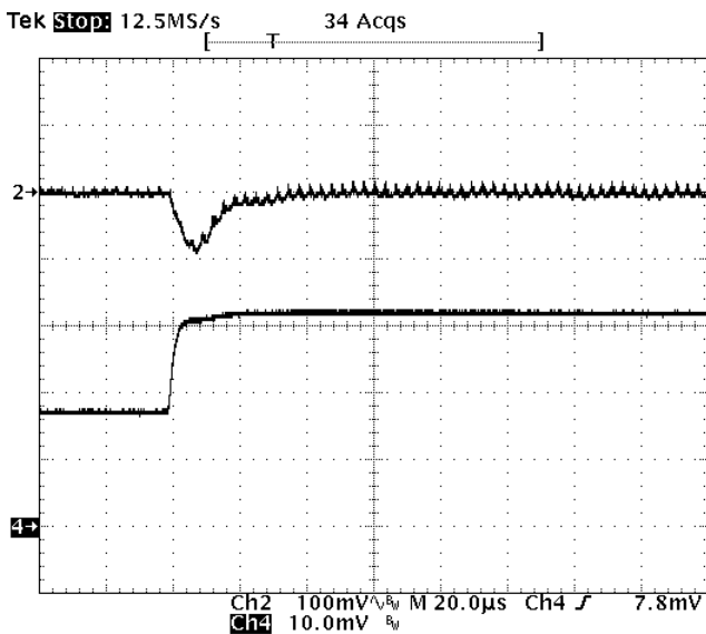
Fig-1.2V-6: Output voltage response for V_{out}=1.2V to positive load current step change from 8A to 16A with slew rate of 5A/\mu s at V_{in}=12V . C_o=47\mu F \times 4 ceramic. Top trace: output voltage (100mV/div.) Bottom trace: load current (5A/div.) Time scale: 20us/div.
