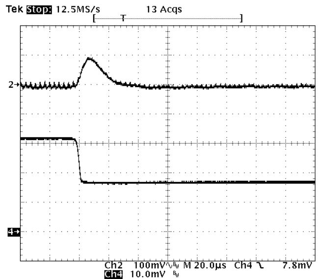
Fig-1.2V-7: Output voltage response for V_{out}=1.2V to negative load current step change from 16A to 8A with slew rate of -5A/\mu s at V_{in}=12V . C_o=47\mu F \times 4 ceramic. Top trace: output voltage (100mV/div.) Bottom trace: load current (5A/div.) Time scale: 20us/div.
