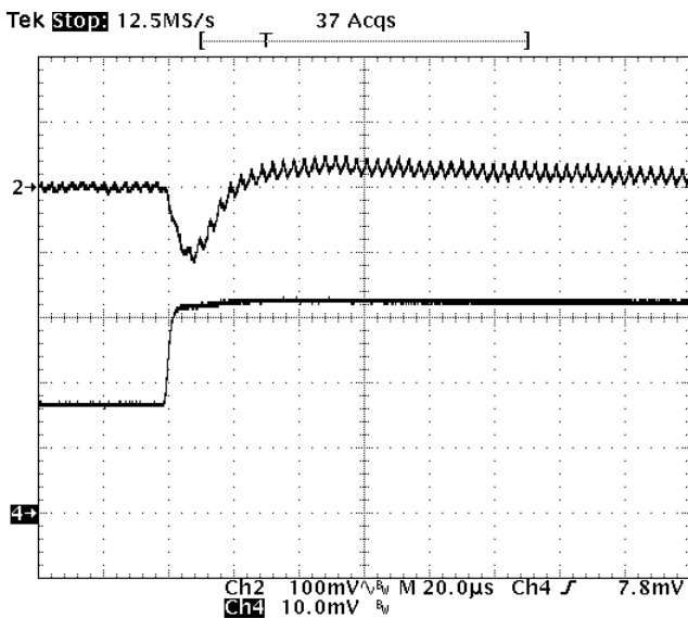
Fig-2.5V-6: Output voltage response for V_{out}=2.5V to positive load current step change from 8A to 16A with slew rate of 5A/\mu s at V_{in}=12V . C_o=47\mu F \times 4 ceramic. Top trace: output voltage (100mV/div.) Bottom trace: load current (5A/div.) Time scale: 20us/div.
