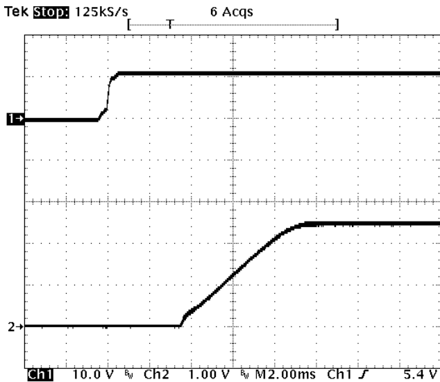
Fig-2.5V-4: Turn-on transient for V_{out}=2.5V with application of V_{in} at full rated load current (resistive) and 47\mu F \times 4 external capacitance at V_{in}=12V . Top trace: V_{in} (10V/div.) Bottom trace: output voltage (1V/div.) Time scale: 2 ms/div.
