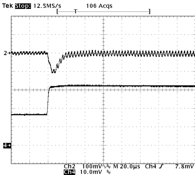
Fig-3.3V-6: Output voltage response for V_{out}=3.3V to positive load current step-change from 8A to 16A with slew rate of 5A/us at V_{in}=12V . C_o=47uF \times 4 ceramic. Top trace: output voltage (100mV/div.) Bottom trace: load current (5A/div.) Time scale: 20us/div.
