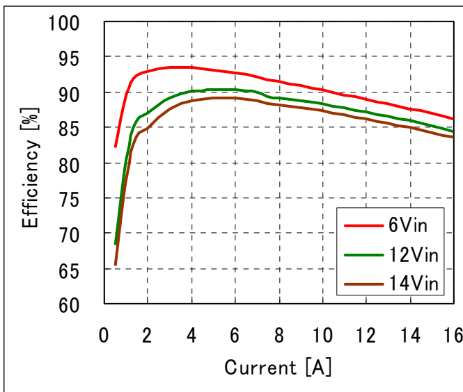
Fig-1.5V-2: Efficiency vs. load current and input voltage for Vout=1.5V. Airflow rate=200 LFM (1m/s) and Ta=25°C.
