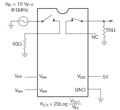
K_{CR} = 20 \log \frac{V_{OUT}}{V_{IN}} Crosstalk
