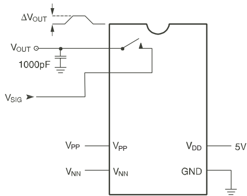
Q = 1000pF \times \Delta V_{OUT}
