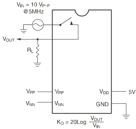
K_O = 20 \log \frac{V_{OUT}}{V_{IN}}
