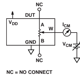
Figure 37. Common-Mode Leakage Current
