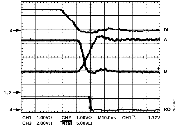
Figure 28. Driver/Receiver Propagation Delays High to Low ( R_{L\text{Diff}} = 54 \Omega , C_{L1} = C_{L2} = 100 \text{ pF} )
