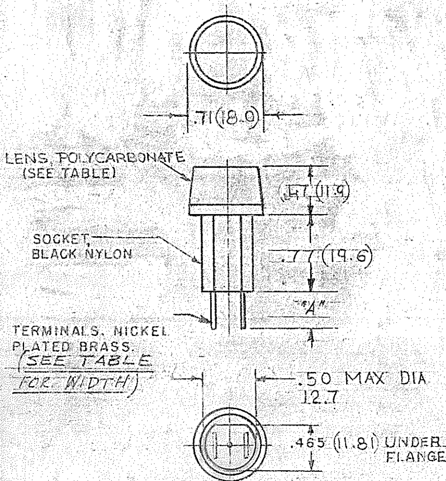
3040 SERIES - ROUND LENS
