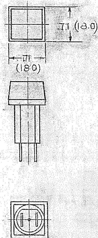
3040 SERIES - SQUARE LENS
