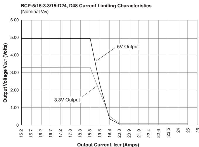
Figure 2. Current Limiting Characteristics
